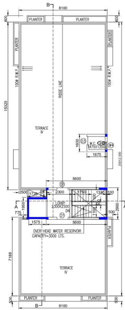
ROOF PLAN
